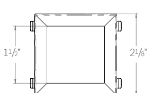
ED1-STL SQUARE TRIMLESS Trimless Style for use with SAIC models only.
